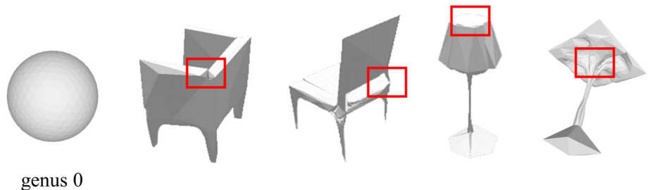
FIGURE 10 Compared to the state-of-art single shaded image-based shape reconstruction method NMR. 8 The results of NMR are lack of concave features, while ours show more accurate and detailed surface structures
