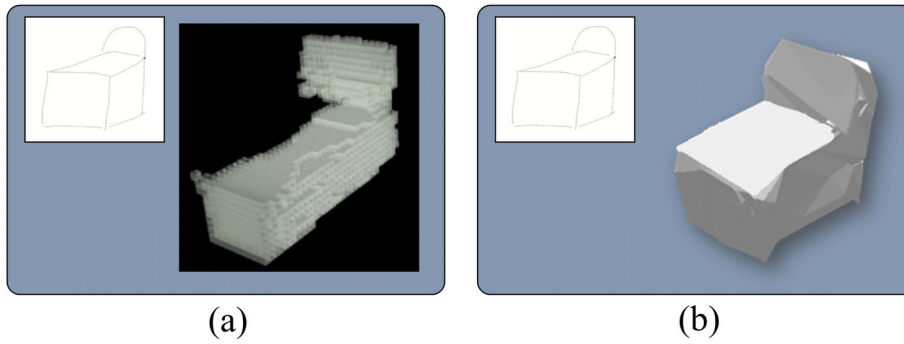
FIGURE 7 Compared to the voxel-based approach. (a) is the voxel-based method 18 and (b) is our method
