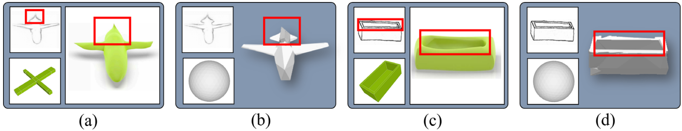
FIGURE 8 Compared to the previous single-view approach. Though the method of Smirnov et al. 16 (a and c) using single sketch as input while specific shapes of template are required for different categories. Our approach (b and d) only needs a sphere as the template for all categories, and recovers more sharp and accurate features as the areas marked by the red boxes above
